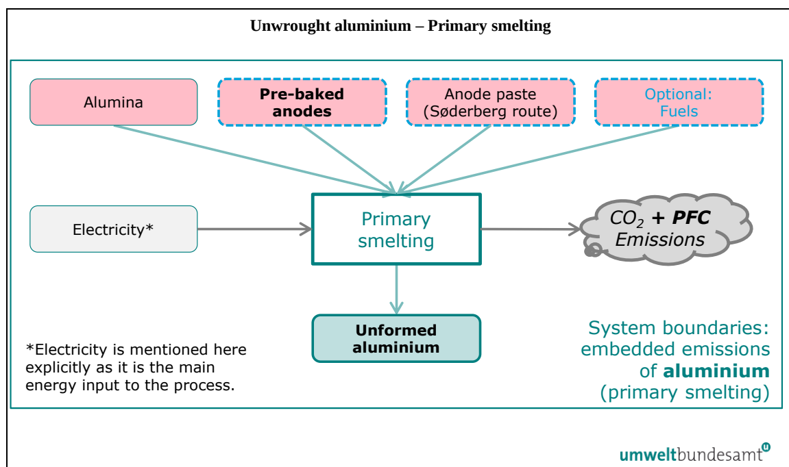
Figure 5-15: System boundaries of the unwrought aluminium – primary smelting production route
