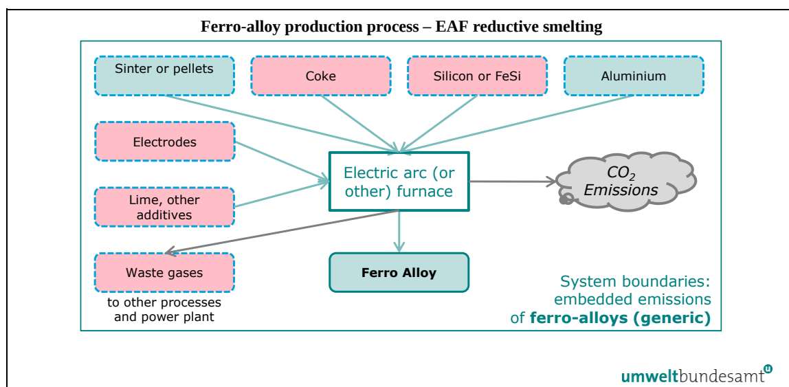
Figure 5-7: System boundaries of Ferro-alloy production processes.
