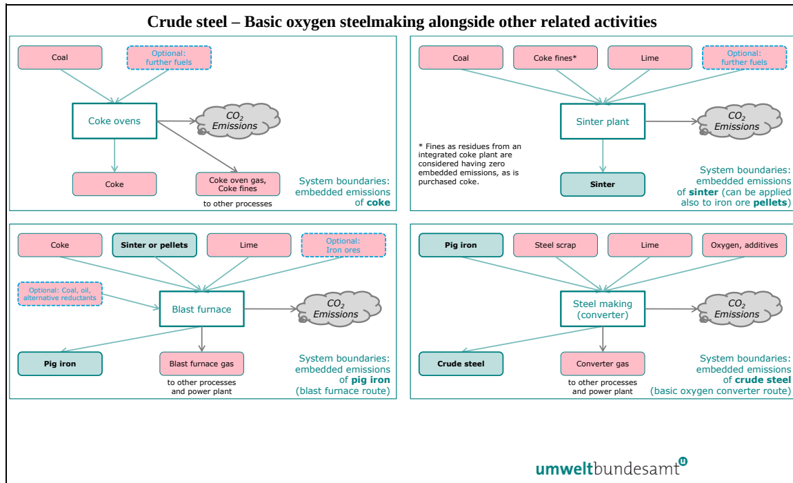
Figure 5-11: System boundaries of basic oxygen steelmaking and related processes.
