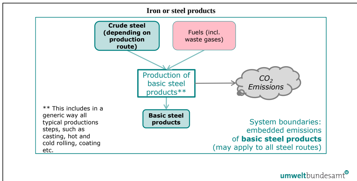
Figure 5-13: System boundaries of steel products production process
