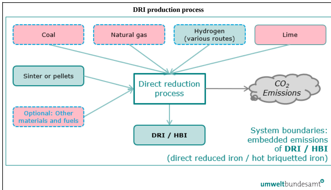
Figure 5-10: System boundaries of the DRI production process
